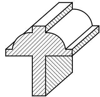
1-1/4" Muntin Bar Profile
