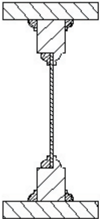
Sash in 4-9/16" Frame Cross Section
